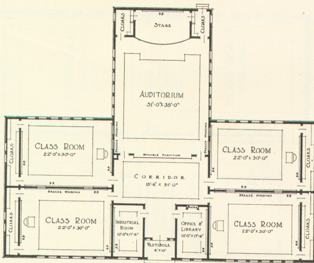
FLOOR PLAN NO 4 FOUR TEACHER COMMUNITY SCHOOL TO FACE EAST OR WEST ONLY
